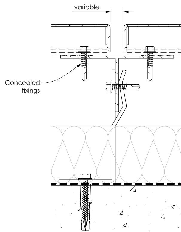
Section Y - Y Vertical Joint Detail (Scale 1 : 2)
