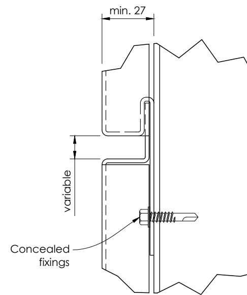
Detail X Horizontal Joint Detail (Scale 1 : 2)
