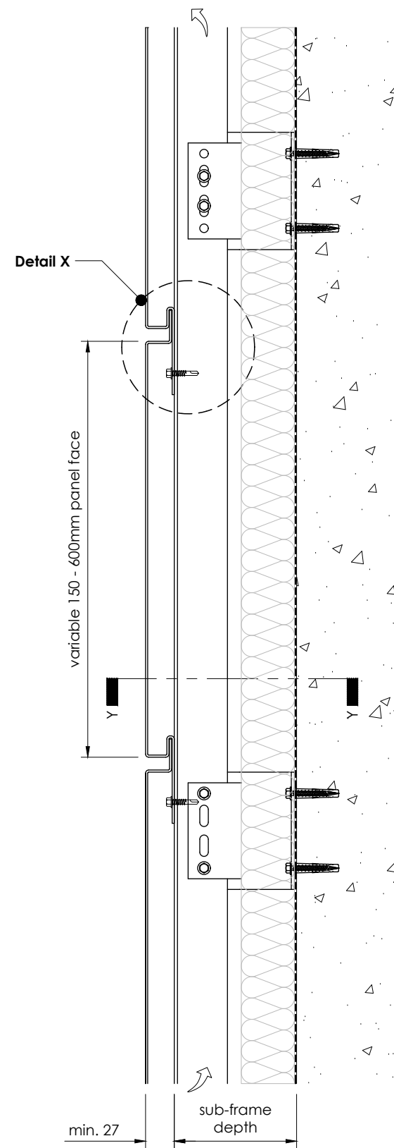
Typical Horizontal Panel Section (Scale 1 : 5)
